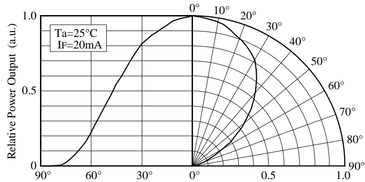
■ Directivity (NSHU550A)
