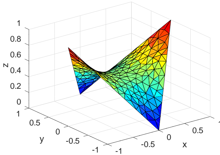
Figure 39: A minimal surface
