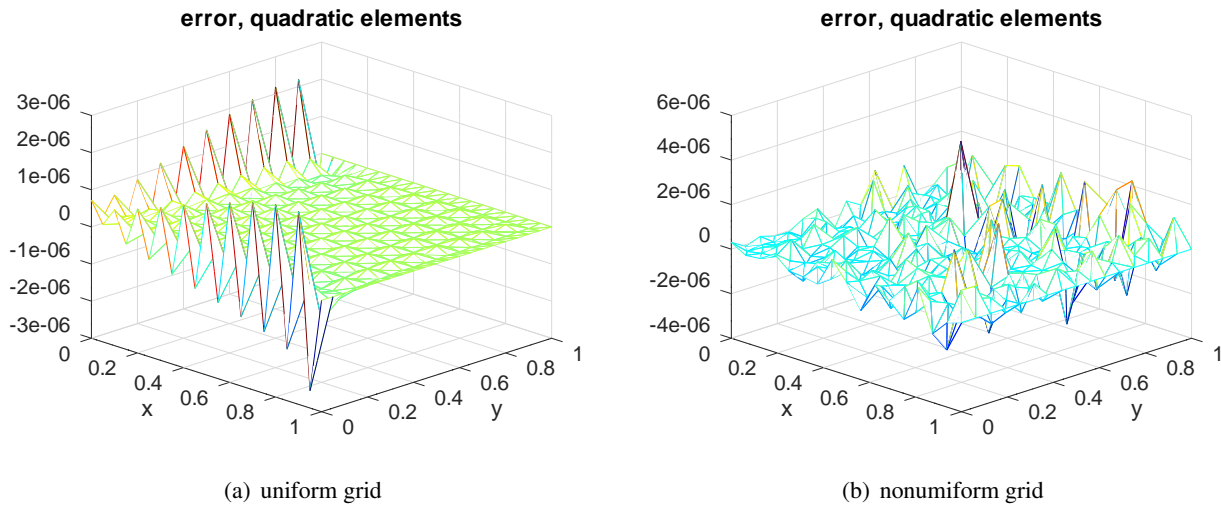
Figure 31: Difference to the exact solution of a BVP
