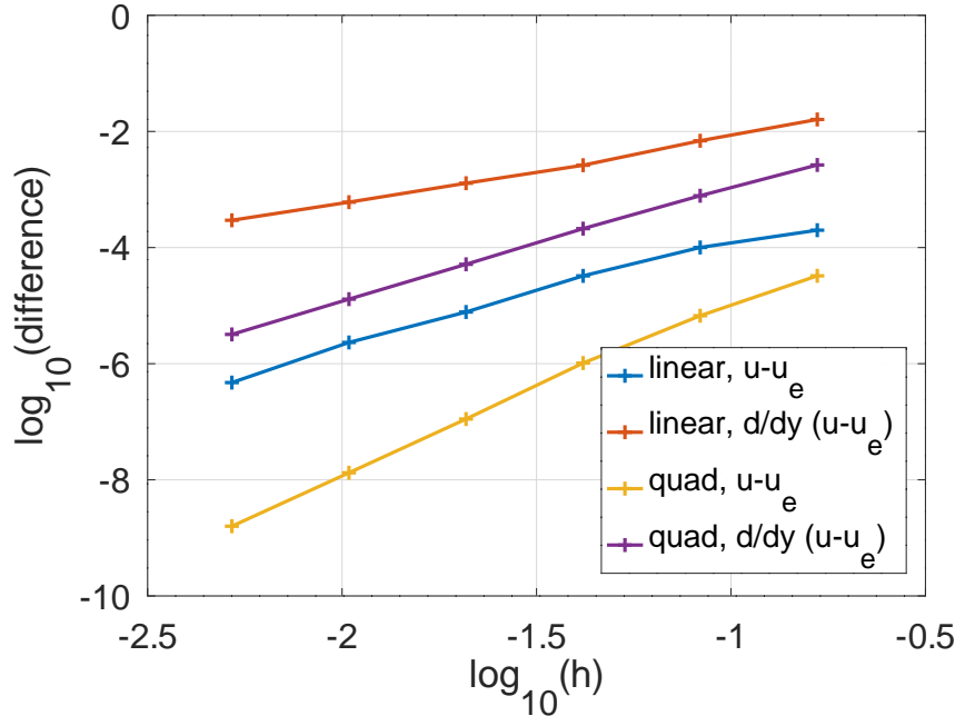
Figure 12: Convergence results for linear and quadratic elements
