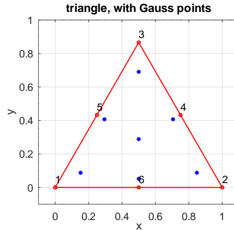
Figure 15: An equilateral, quadratic triangle, the Gauss integration points and the element stiffness matrix
