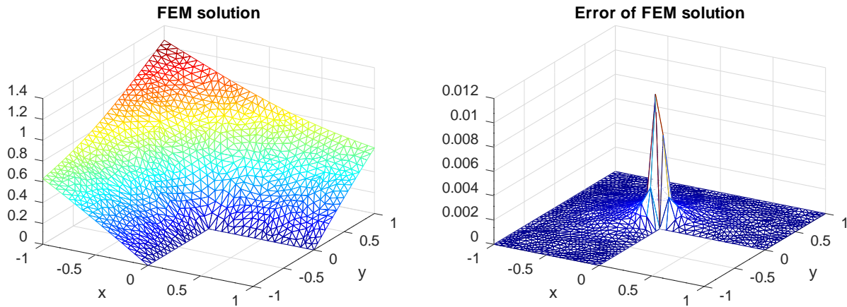
Figure 35: A solution with singular partial derivatives at the origin
