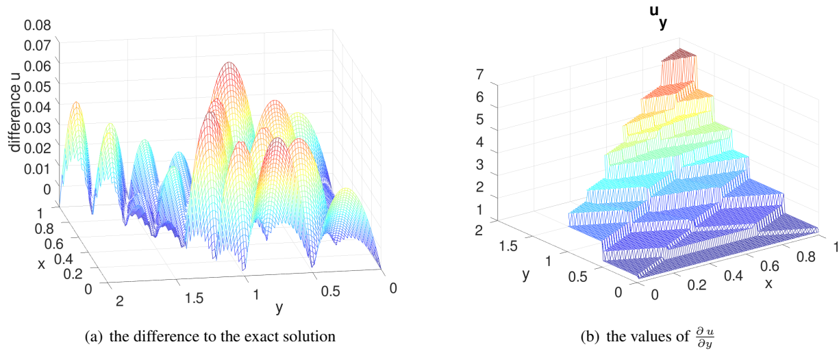
Figure 20: Difference to the exact solution and values of \frac{\partial u}{\partial y} , using a first order mesh
