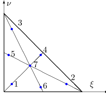
Figure 26: Gauss integration of order 5 on the standard triangle, using 7 integration points
