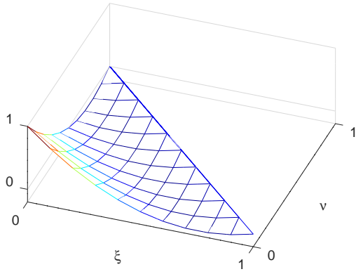
(a) \Phi_1(\xi, \nu) = (1 - \xi - \nu)(1 - 2\xi - 2\nu)
