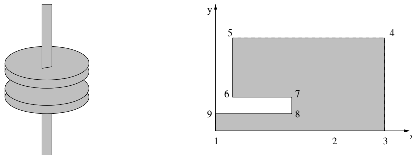
Figure 40: The capacitance and the section used for the modeling
