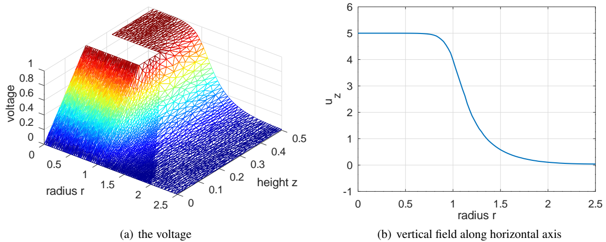
Figure 43: Voltage plot and electric field between the plates of the capacitance
