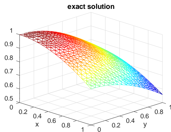
Figure 30: The radial Bessel function as solution of a BVP
