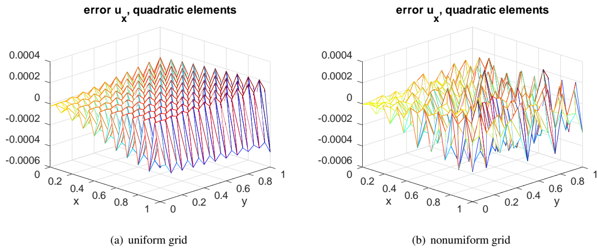
Figure 33: Difference of \frac{\partial u}{\partial x} to the exact solution, using second order elements
