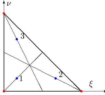
Figure 25: Gauss integration of order 2 on the standard triangle, using 3 integration points
