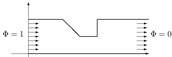
Figure 37: Fluid flow between two plates, the setup
