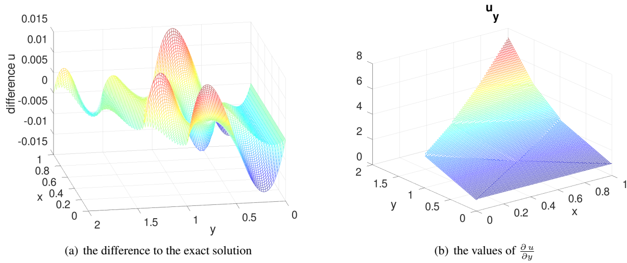
Figure 21: Difference to the exact solution and values of \frac{\partial u}{\partial y} , using a second order mesh
