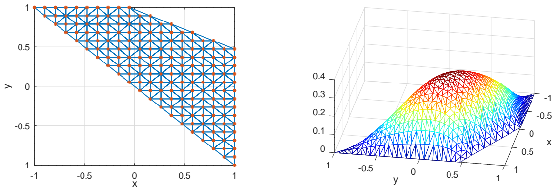
Figure 10: A mesh generated by a Delaunay triangulation and the solution of a BVP
