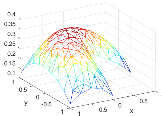
Figure 4: Solution of a diffusion problem on a L-shaped domain
