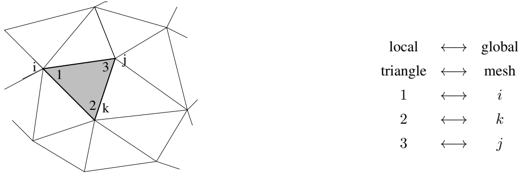
Figure 27: Local and global numbering of nodes
