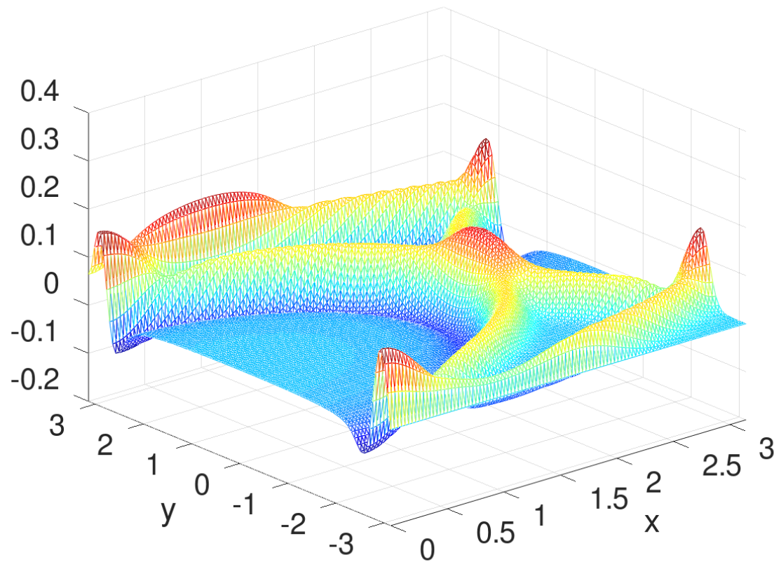
Figure 29: Traveling waves on a rectangle
