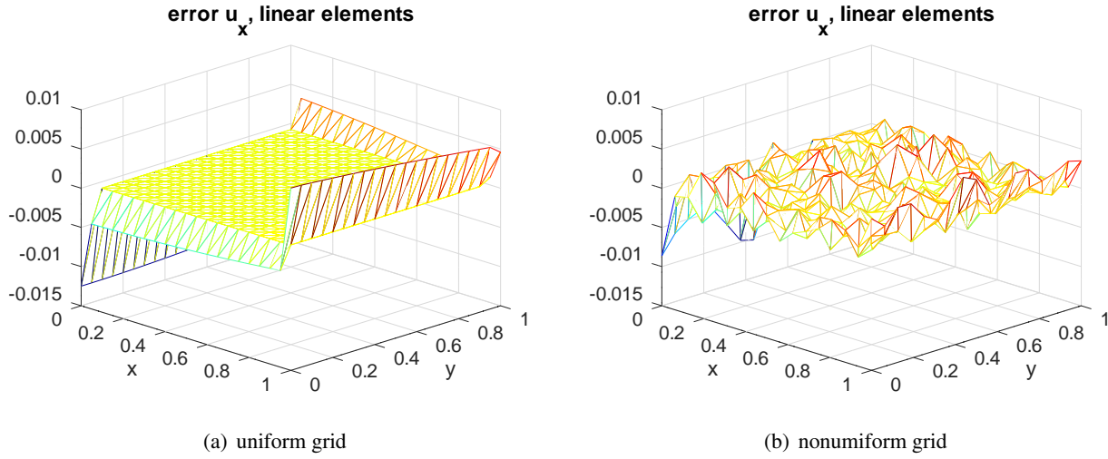
Figure 34: Difference of \frac{\partial u}{\partial x} to the exact solution, using first order elements
