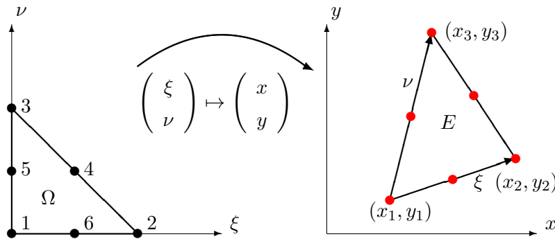
Figure 24: Transformation of standard triangle to general triangle
