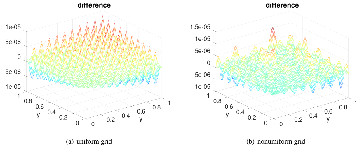
Figure 32: Difference to the exact solution of a BVP, using quadratic elements and interpolation to a finer grid.
