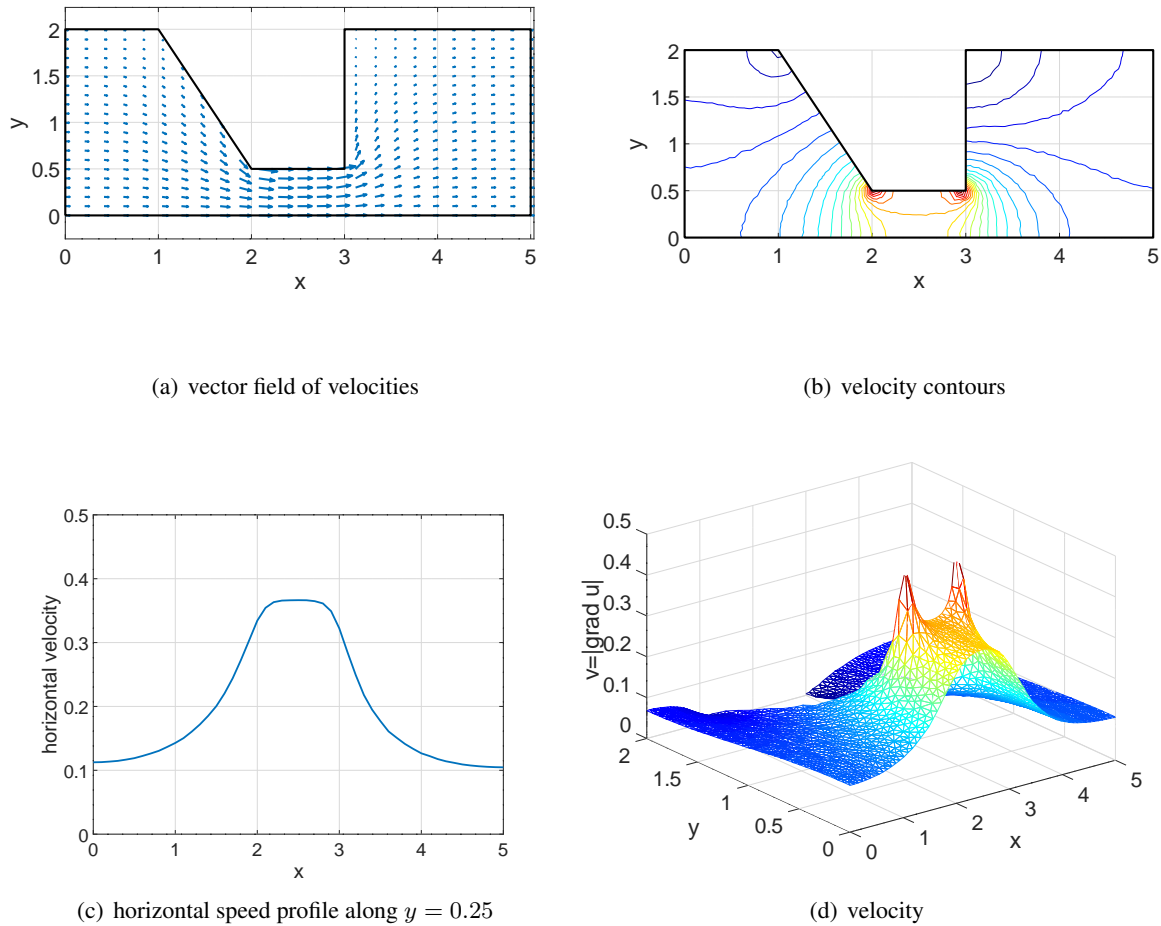
Figure 38: Velocity field of an ideal fluid, full view and details
