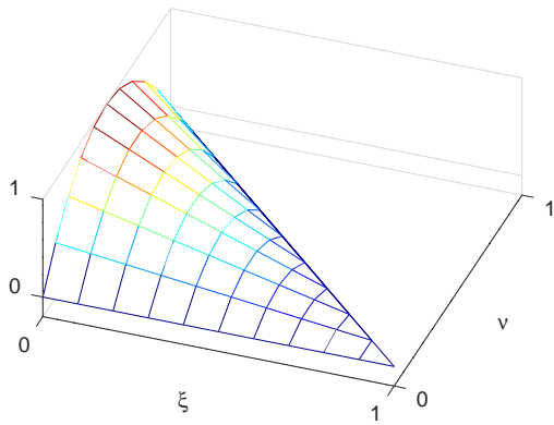
(e) \Phi_5(\xi, \nu) = 4\nu(1 - \xi - \nu)
