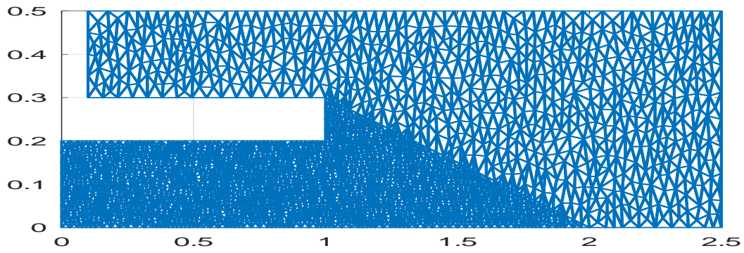
Figure 41: A mesh on the domain
