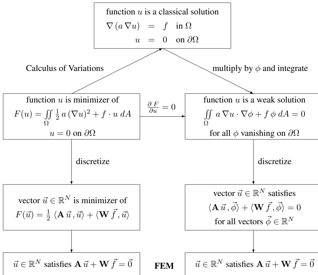
Figure 23: Classical and weak solutions, minimizers and FEM
