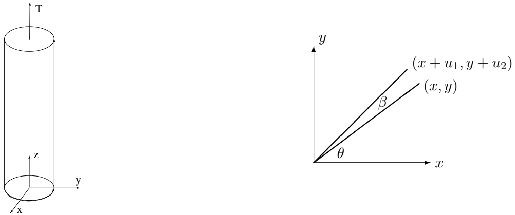
Figure 44: Torsion of a shaft
