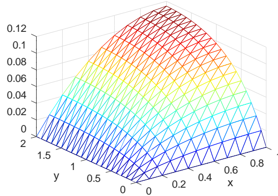
Figure 2: Solution of -\Delta u = 0.25 on a rectangle
