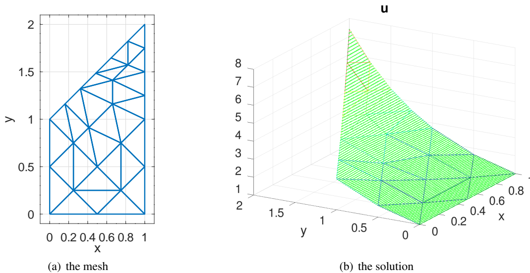
Figure 19: The mesh and the solution for a BVP
