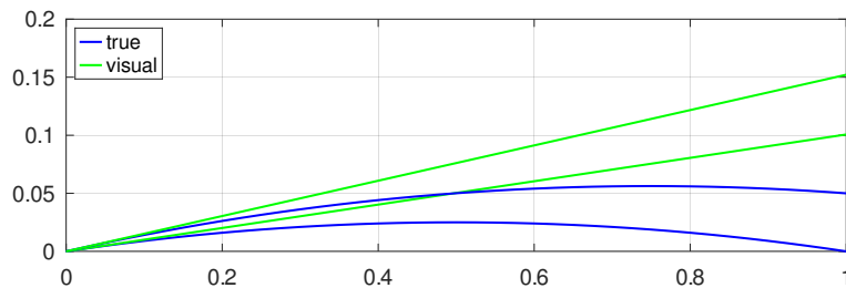
Figure 144: Fata Morgana: how the image of two points appear to the observer
