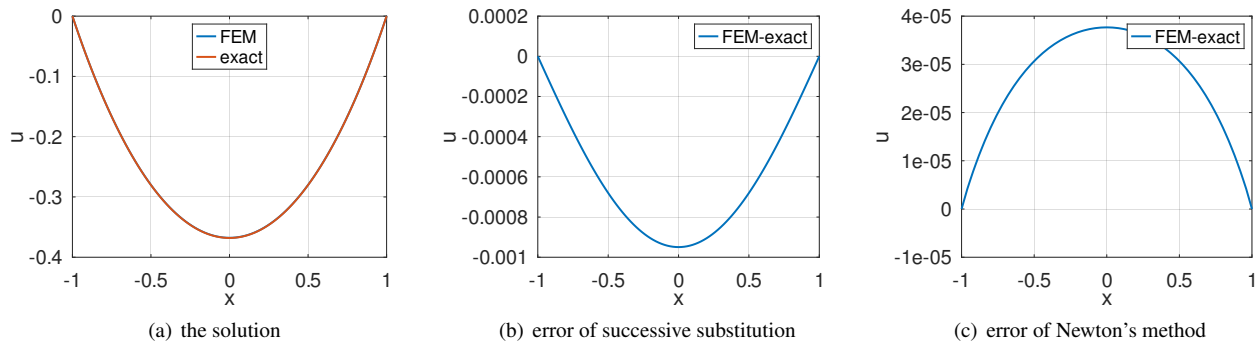
Figure 145: The solution of Keller's boundary value problem and the difference of the approximations by successive substitution and Newton's method
