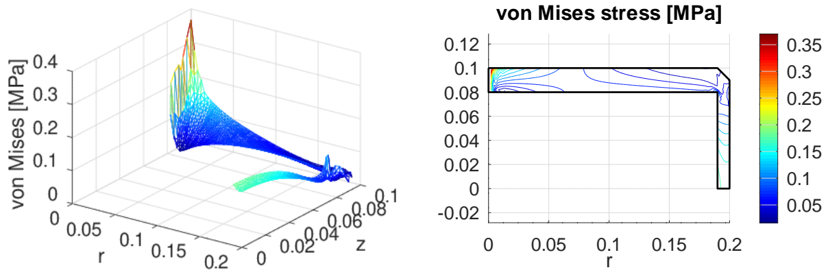
Figure 172: The von Mises stress for the rotating rubber box
