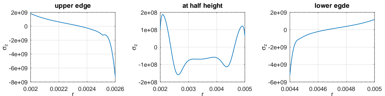
Figure 177: The normal pressures \sigma_z along upper and lower edge and at half height
