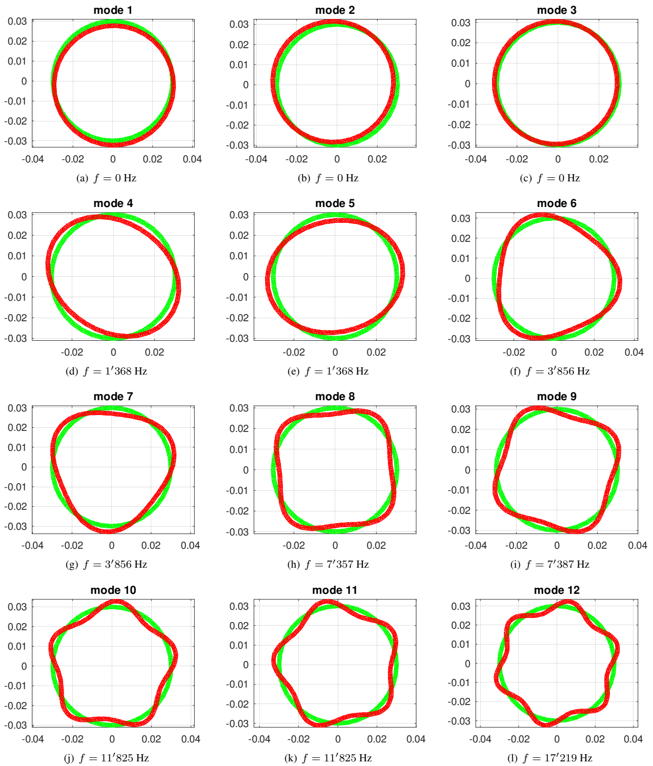
Figure 180: The first twelve eigen modes of a vibration ring
