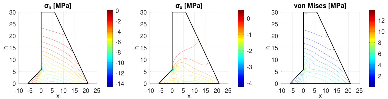
Figure 178: The normal stresses and the von Mises stress in a water dam
