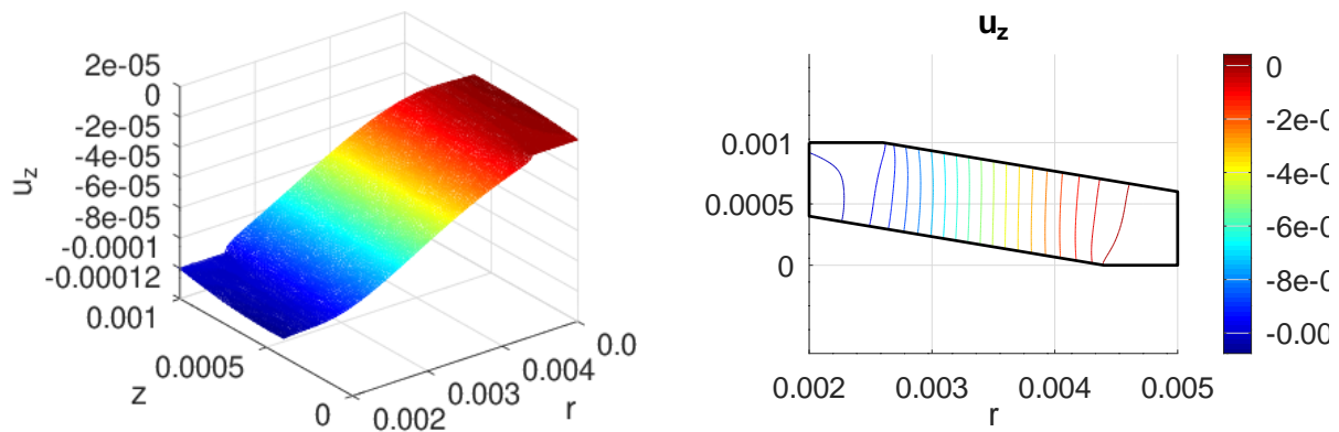
Figure 175: The height displacement u_z
