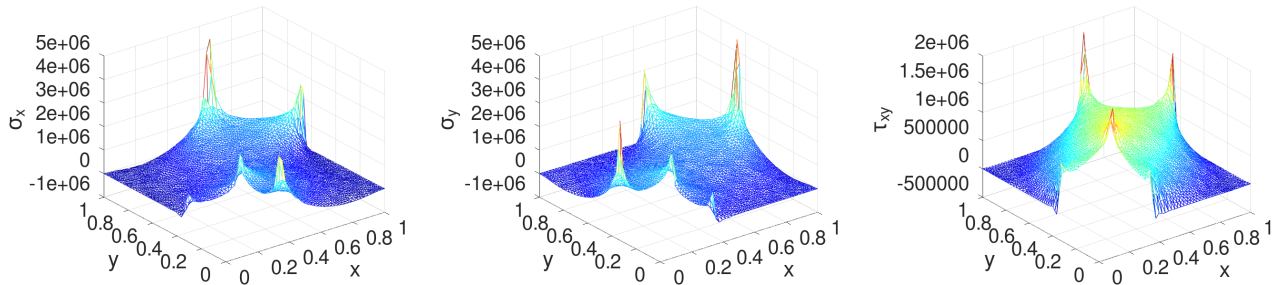
Figure 159: The stresses for a plane stress example
