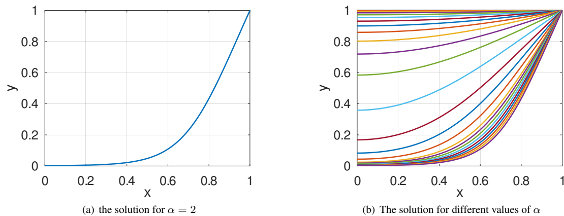
Figure 155: A BVP describing mass transfer in a porous catalyst, second setup
