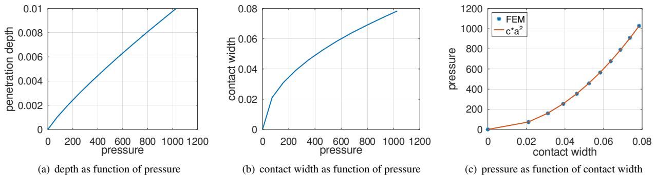
Figure 186: Contact with cylinder: results of pressure and contact width for small penetration depth
