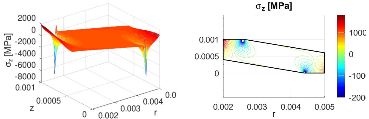
Figure 176: The normal stress \sigma_z
