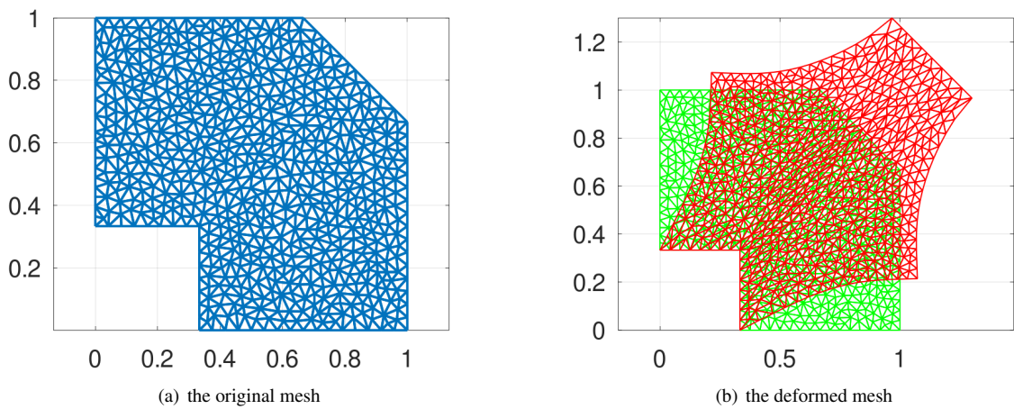
Figure 157: The original and deformed Mesh for a plane stress example
