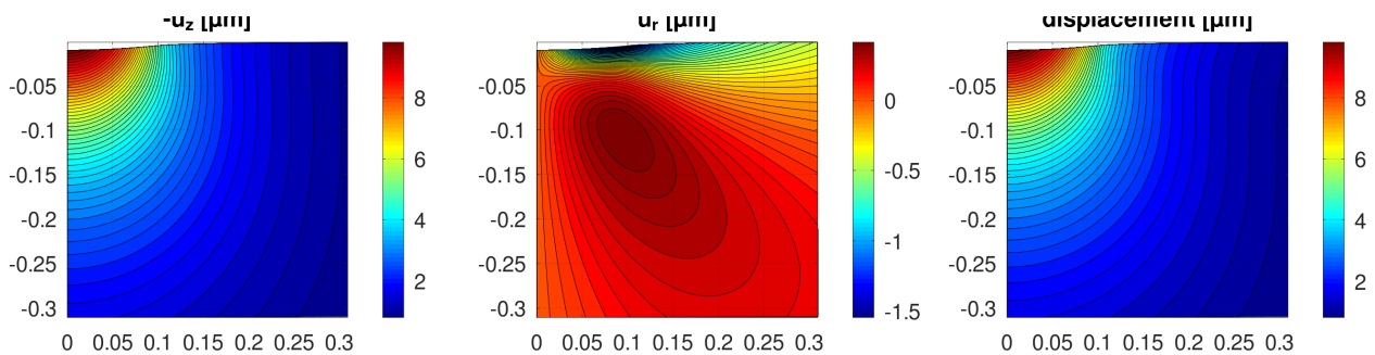
Figure 189: Contact with sphere: contours for the displacements u_z and u_r and \sqrt{u_r^2 + u_z^2}
