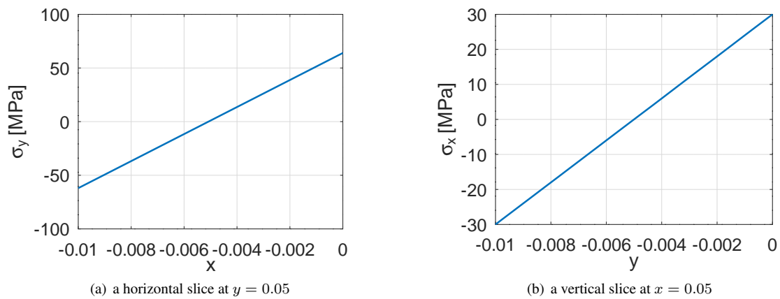
Figure 165: A horizontal slice with \sigma_y shown and a vertical slice with \sigma_x shown
