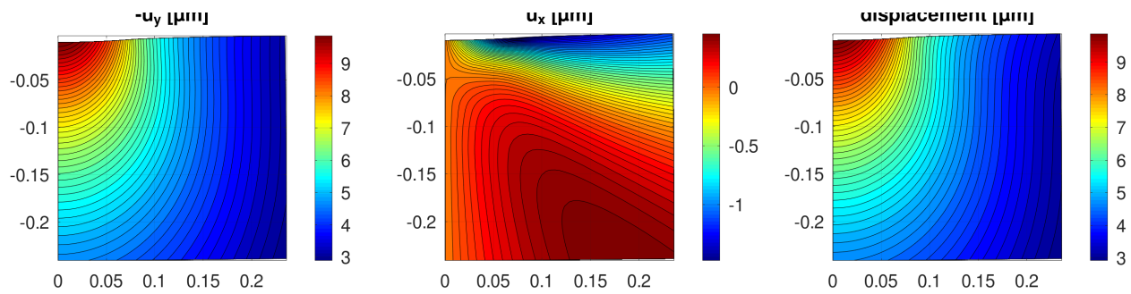
Figure 184: Contact with cylinder: contours for the displacements u_2 and u_1 and \sqrt{u_1^2 + u_2^2}
