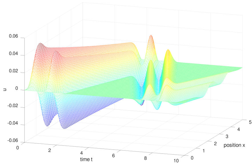
Figure 156: Motion of a string, excited by an initial pulse close to x = 0
