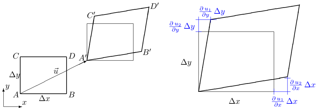
Figure 3: Definition of strain: a rectangle before and after deformation
