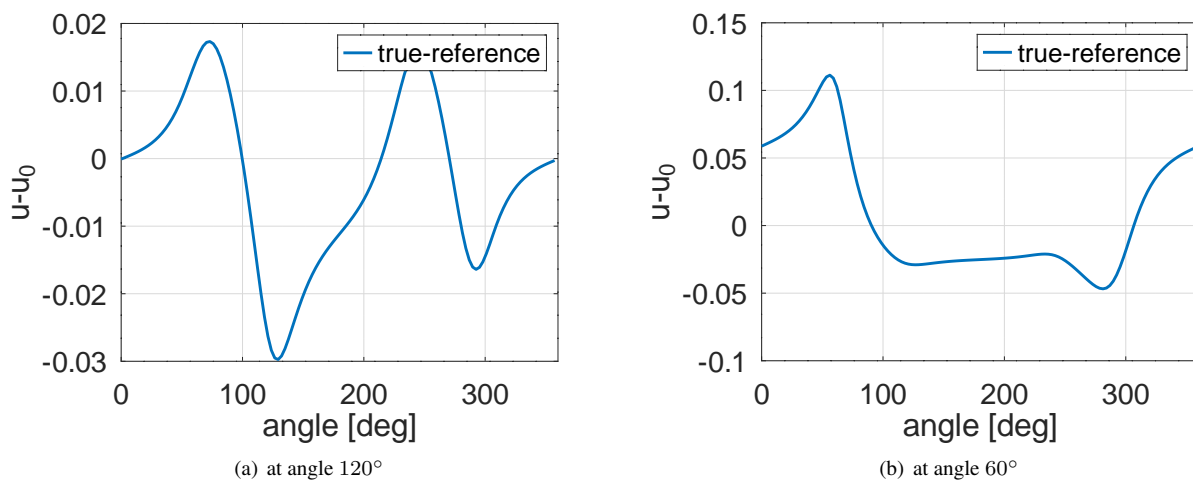
Figure 139: Differences of the voltage and the reference voltage
