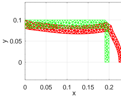
Figure 170: The upper half of the original and deformed domain for the rotating rubber box
