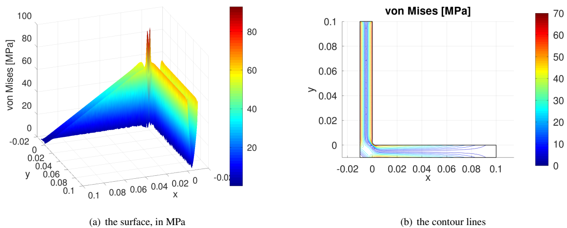
Figure 166: The von Mises stress on the crook, as surface and level curves
