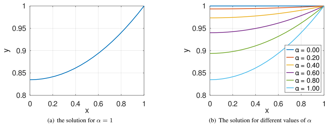
Figure 154: A BVP describing mass transfer in a porous catalyst
