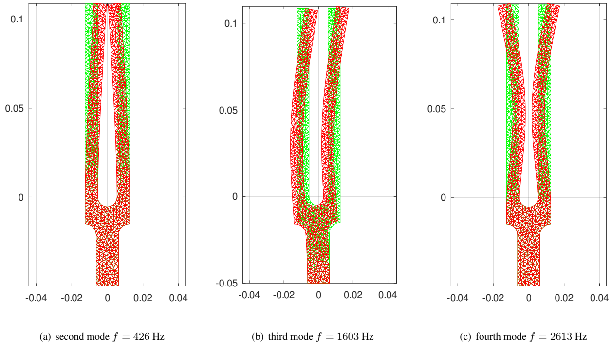
Figure 179: Three eigenmodes of a tuning fork
