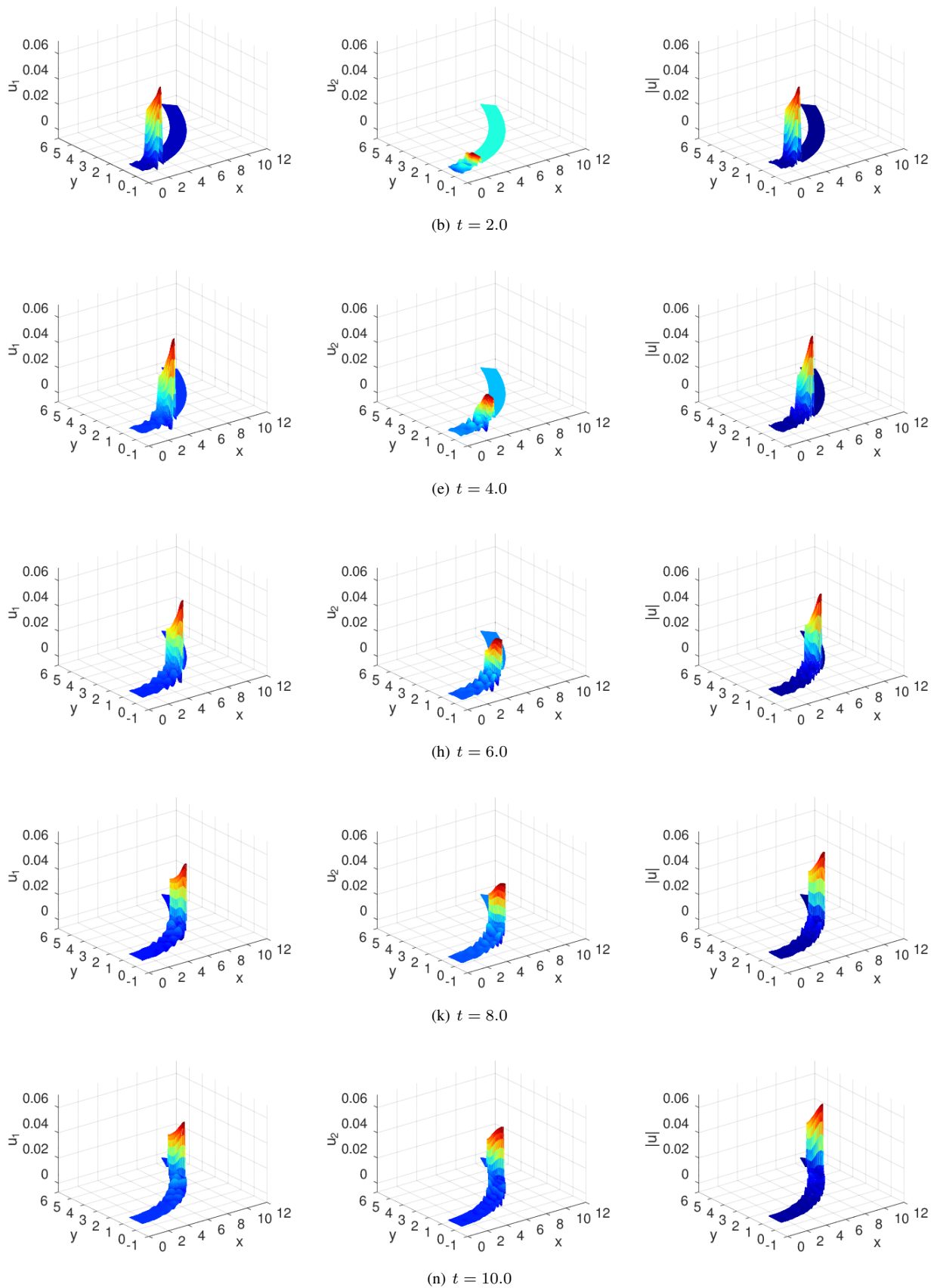
Figure 198: An elastic wave moving in a turn at times 2, 4, 6, 8 and 10. The left column shows the horizontal displacement u_1 , the middle column the vertical displacement u_2 and the column on the right u = \sqrt{u_1^2 + u_2^2} .
