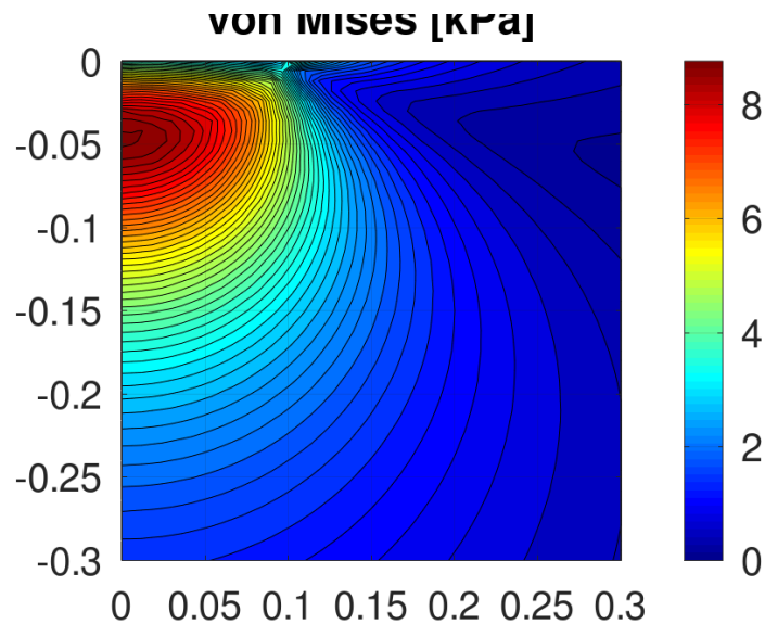
Figure 192: The von Mises stress for a contact with a sphere for given normal pressure \sigma_z(r, 0)
