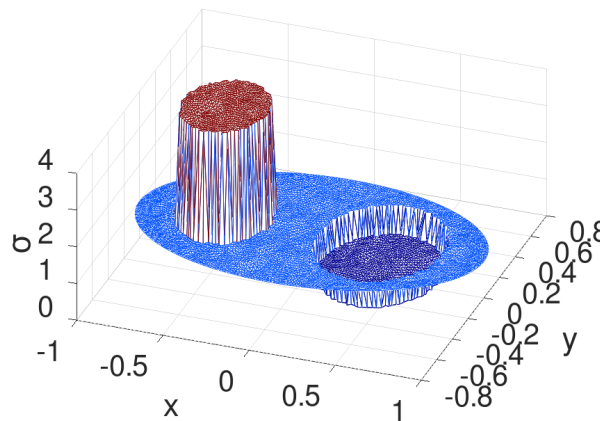
Figure 135: The conductivity with the conducting “heart” on the left and the insulating “lung” on the right
