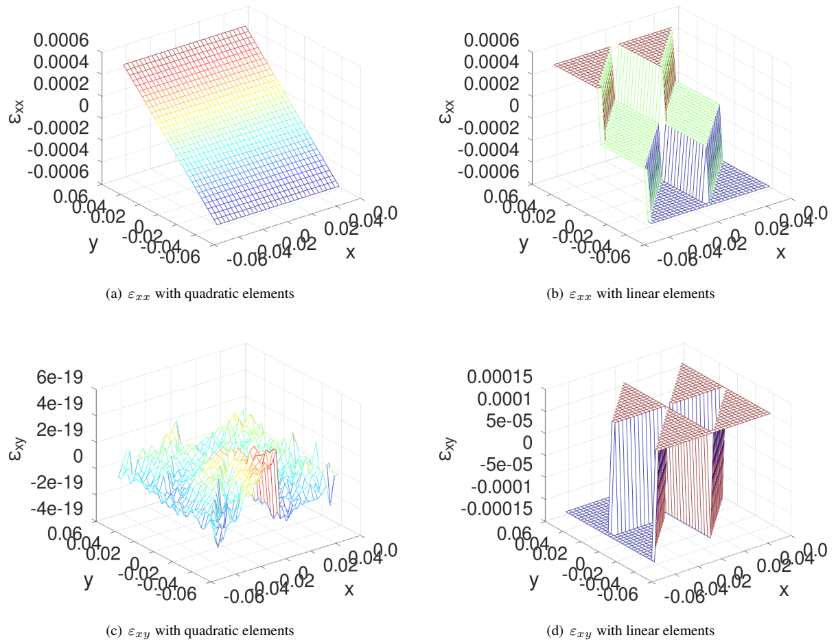
Figure 63: The strains \varepsilon_{xx} and \varepsilon_{xy} with two layers in each direction for linear and quadratic elements
