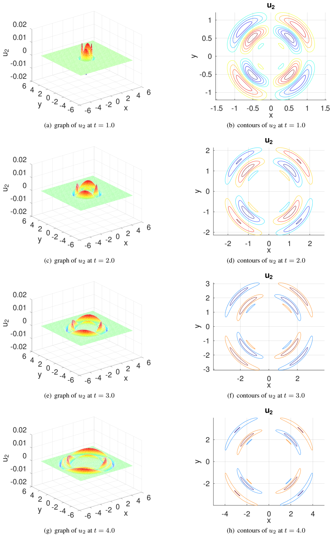
Figure 194: The vertical displacement u_2 of an elastic cylindrical wave
