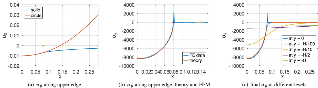
Figure 183: The vertical displacement u_2 along the upper edge and the normal stress \sigma_y at different levels
