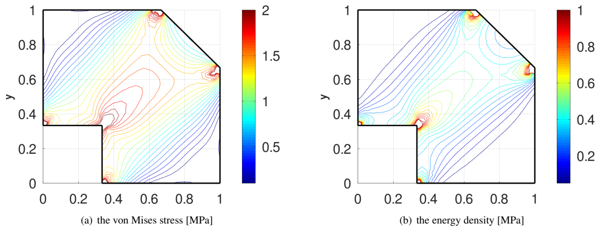
Figure 160: The von Mises stress and the energy density for a plane stress example
