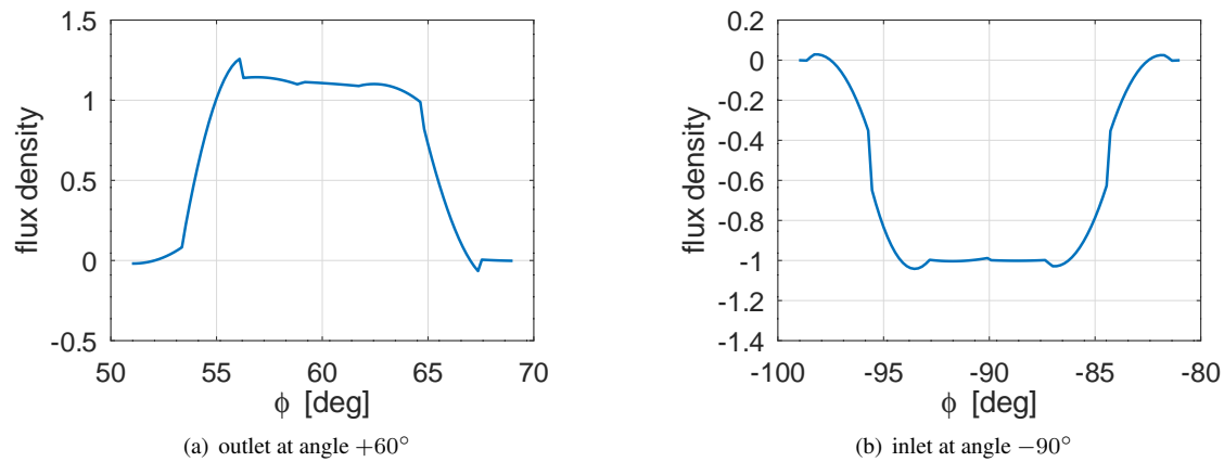
Figure 140: Flux density at inlet and outlet
