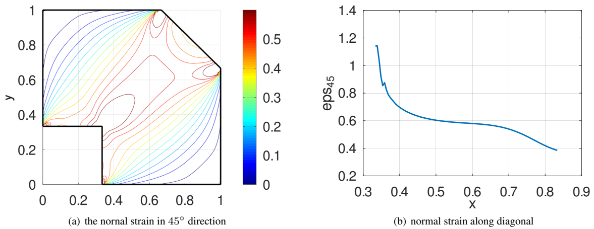
Figure 161: The normal strain in the 45° direction for a plane stress example
