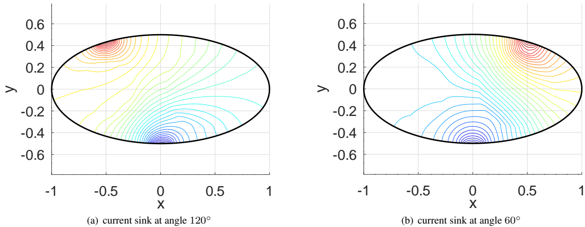
Figure 136: Contours of the voltages
