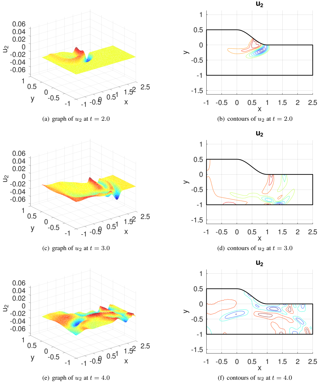
Figure 196: The vertical displacement u_2 of an elastic cylindrical wave
