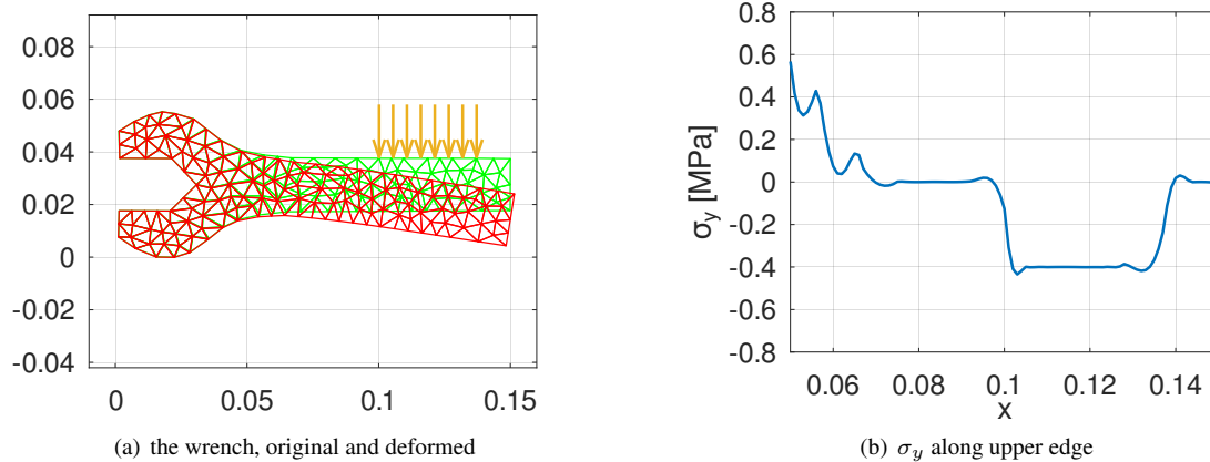
Figure 168: The deformed wrench and the stress \sigma_y along upper edge with the applied load
