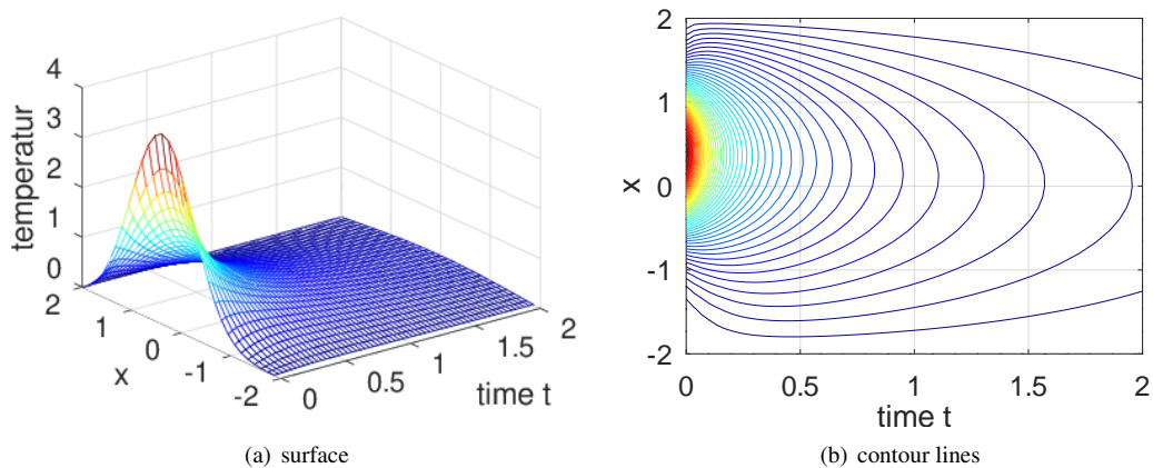
Figure 113: The temperature at different times along y = 0
