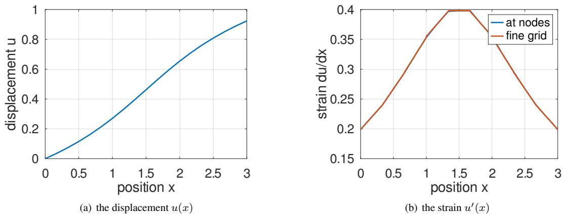
Figure 142: Displacement and strain for a beam with thinner midsection
