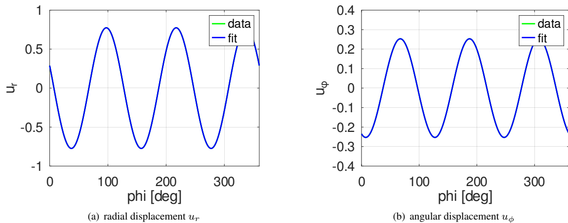
Figure 181: Radial displacement u_r and angular displacement u_\phi for mode 7. Shown are the FEM data and the best fit of the form c_1 + c_2 \cos(n\phi) + c_3 \sin(n\phi) with n = 3 .
