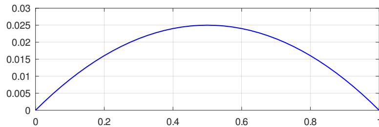
Figure 143: Fata Morgana: the ray of light for a point on the ground
