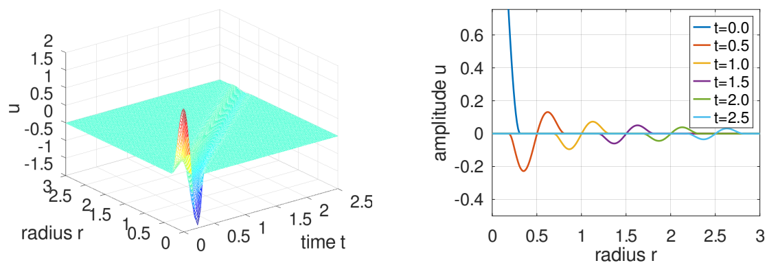
Figure 127: A spherical wave as function of time t and radius r = \sqrt{x^2 + y^2 + z^2}
