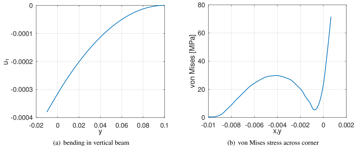
Figure 167: The bending of the centerline of the vertical beam and the von Mises stress on the 45^\circ line through the origin
