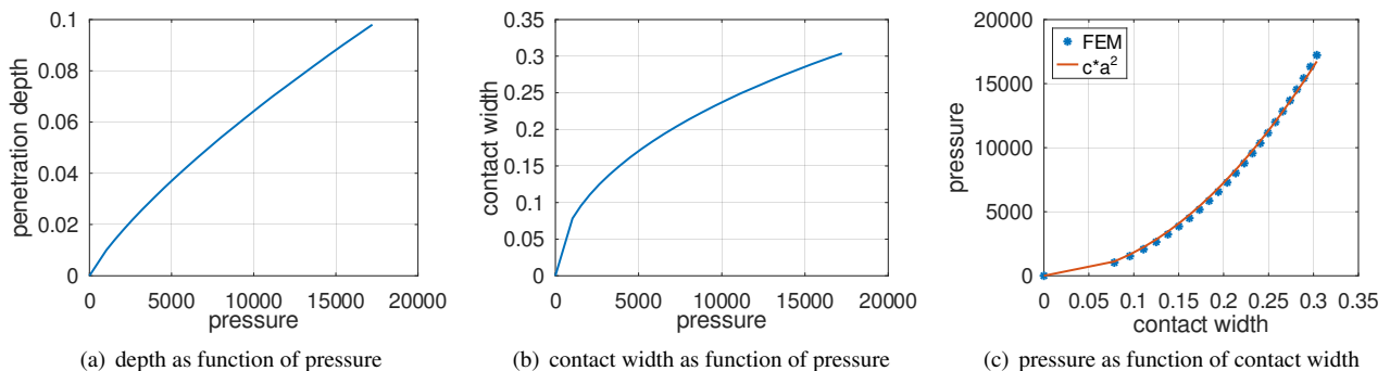
Figure 187: Contact with cylinder: results of pressure and contact width for large penetration depth
