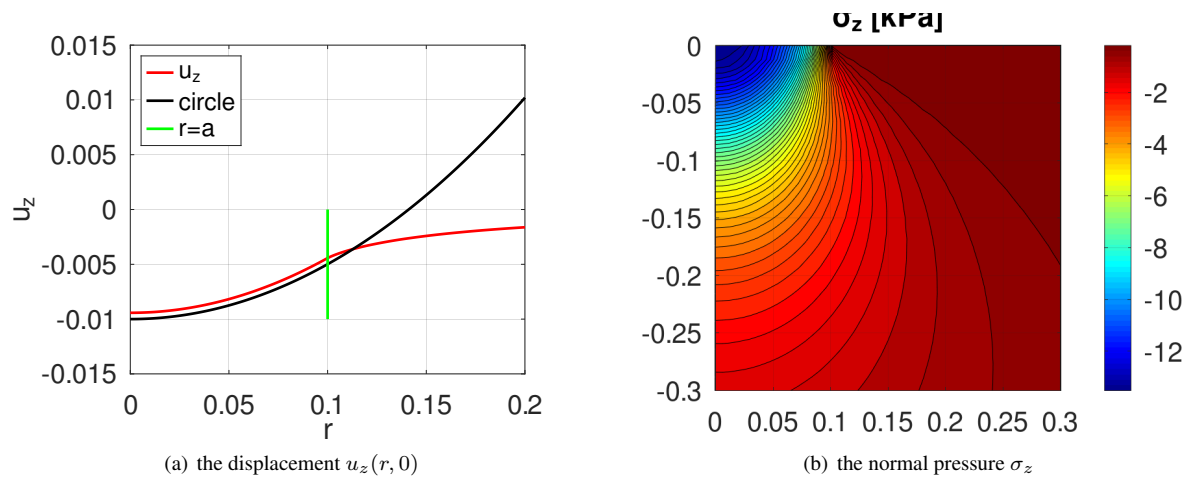
Figure 191: Contact with a sphere for given normal pressure \sigma_z(r, 0)
