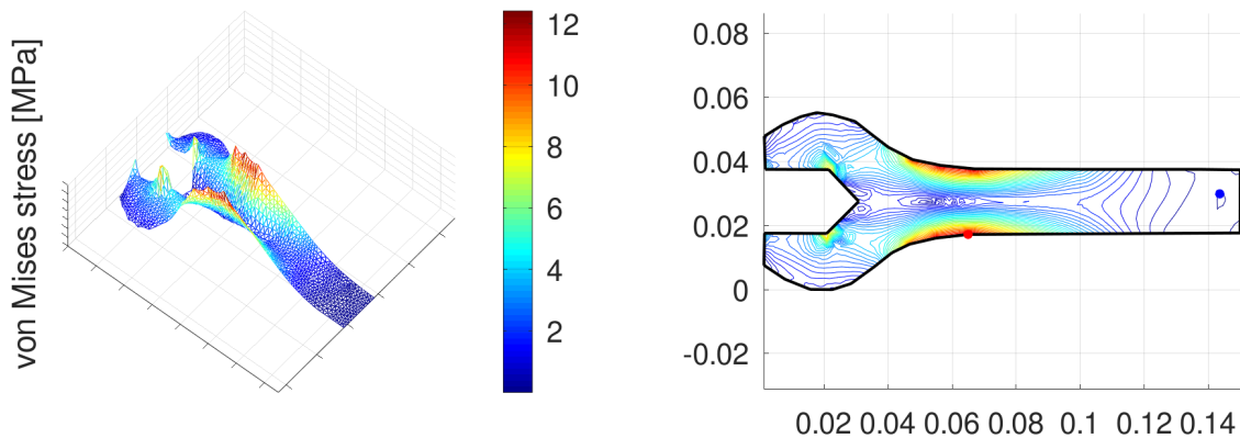
Figure 169: Surface and contour plot of the von Mises stress in [MPa]
