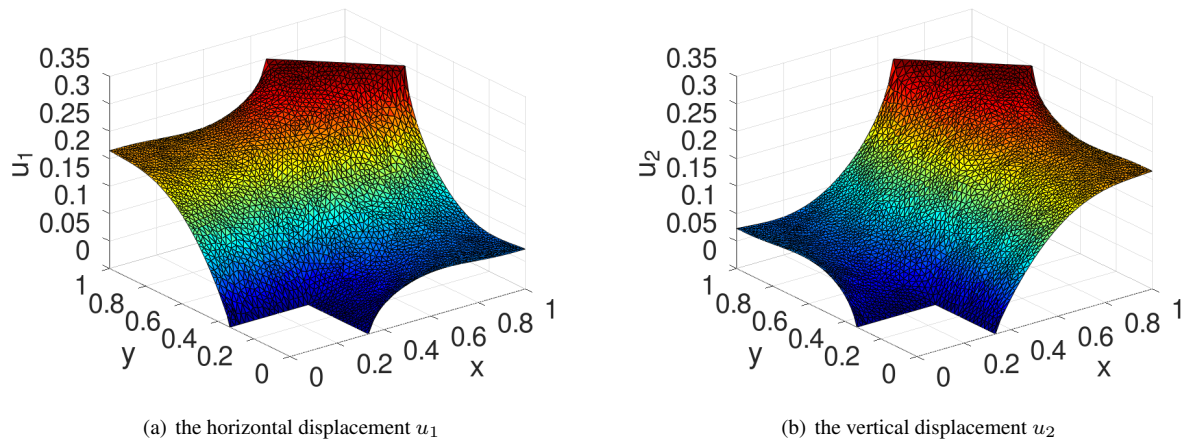
Figure 158: The displacements for a plane stress example
