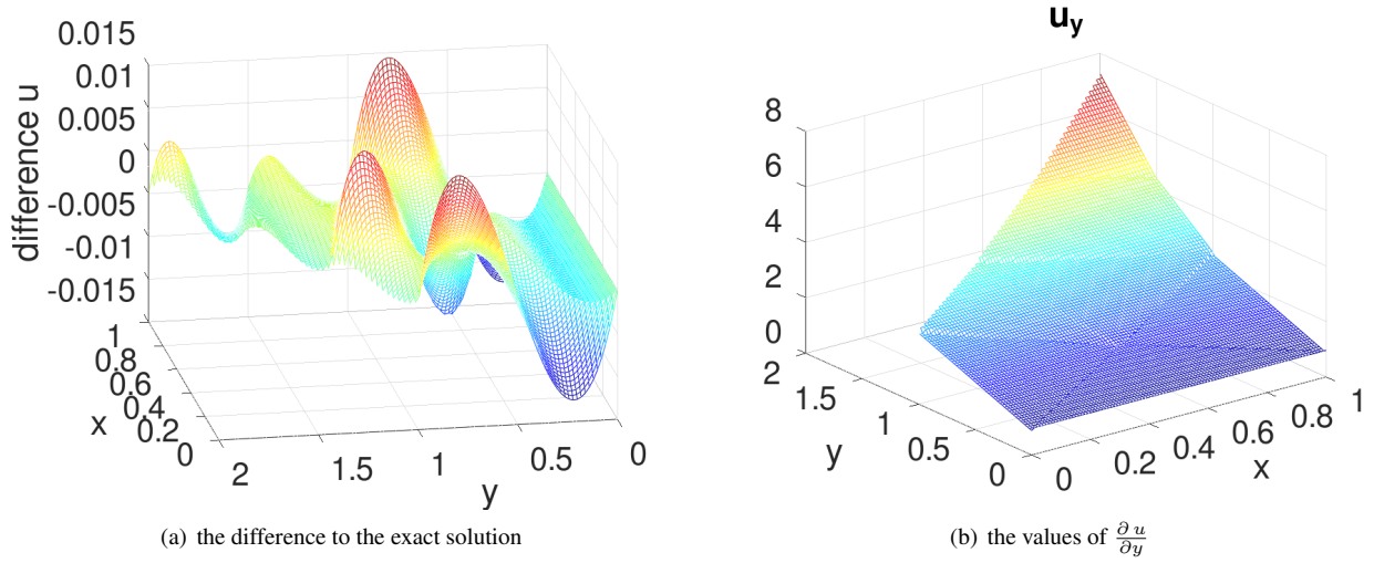
Figure 48: Difference to the exact solution and values of \frac{\partial u}{\partial y} , using a second order mesh
