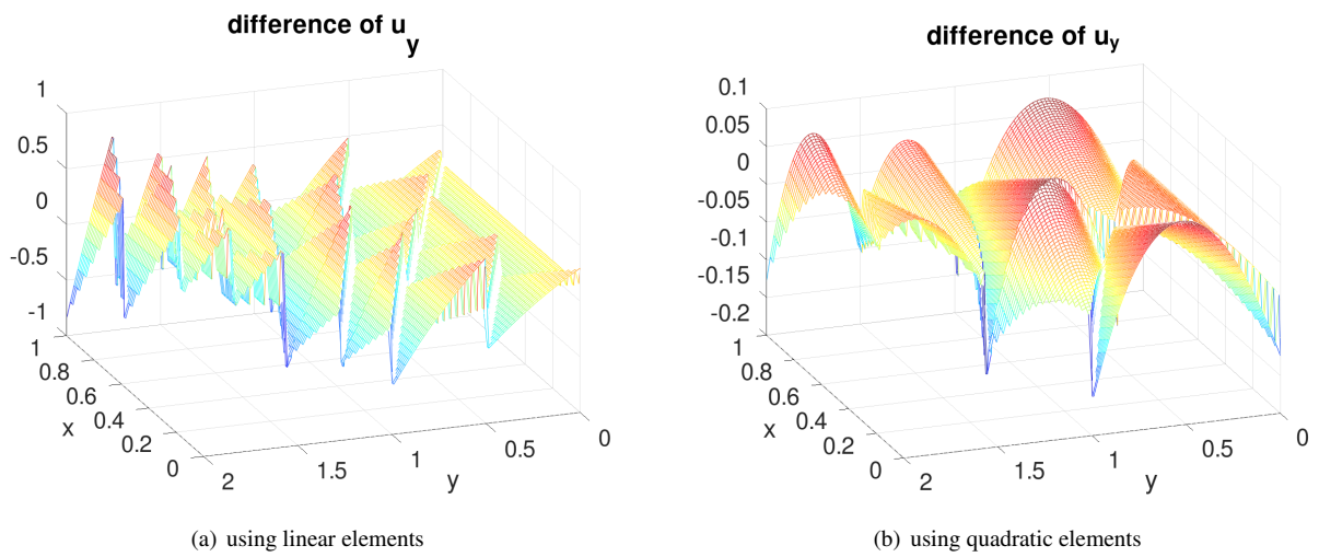
Figure 49: Difference of the approximate values of \frac{\partial u}{\partial y} to the exact values
