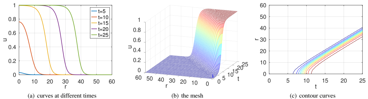
Figure 150: A dynamic solution of Fisher's equation for the radially symmetric setup
