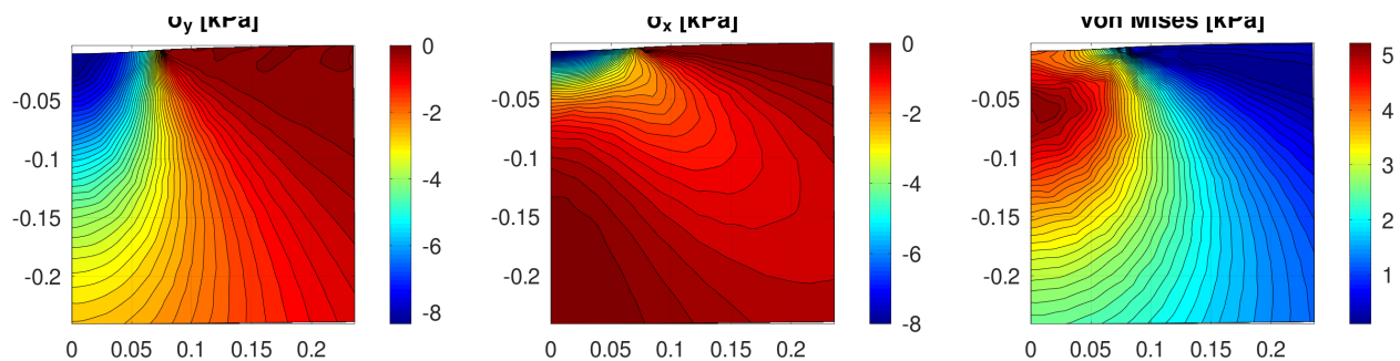
Figure 185: Contact with cylinder: contours for the two normal stresses and the von Mises stress
