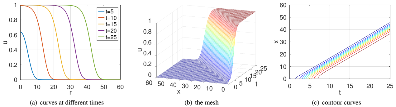
Figure 149: A dynamic solution of Fisher's equation
