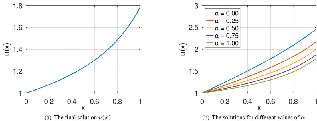
Figure 147: A BVP with multiple nonlinear contributions
