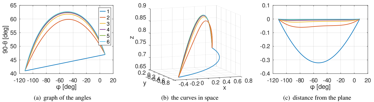
Figure 151: The connections between Salt Lake City and Zürich. The plots of latitude as function of longitude, the curves in space on the earth as sphere with radius 1 and the distances from the plane with the great circle.
