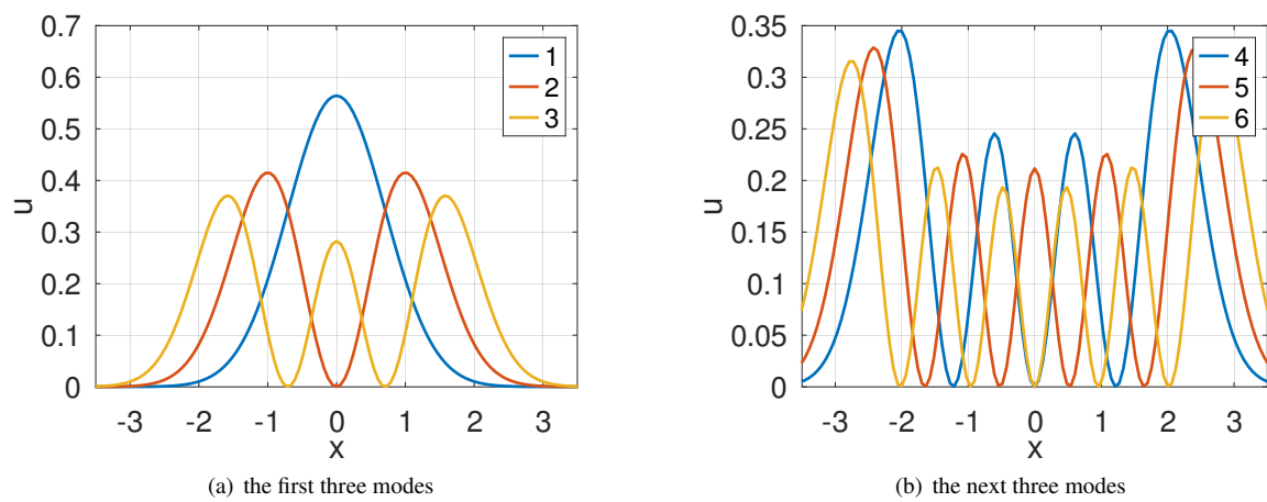
Figure 134: The PDF for the first six modes of the harmonic Schrödinger operator
