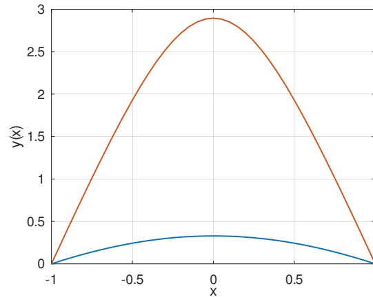
Figure 146: Two solutions of -u''(x) = \frac{1}{2} \exp(u(x)) with u(-1) = u(1) = 0
