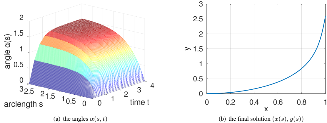
Figure 153: Time evolution and the final solution for a dynamic bending beam
