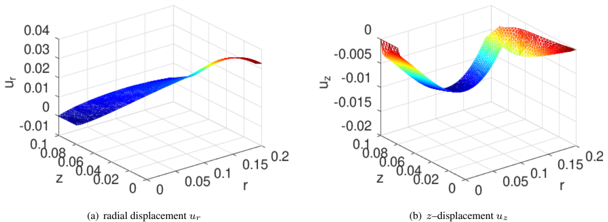
Figure 171: The displacements u_r and u_z for the rotating rubber box
