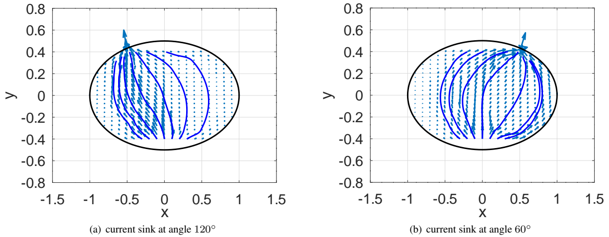
Figure 137: The vector field for the current density \vec{J} and a few streamlines
