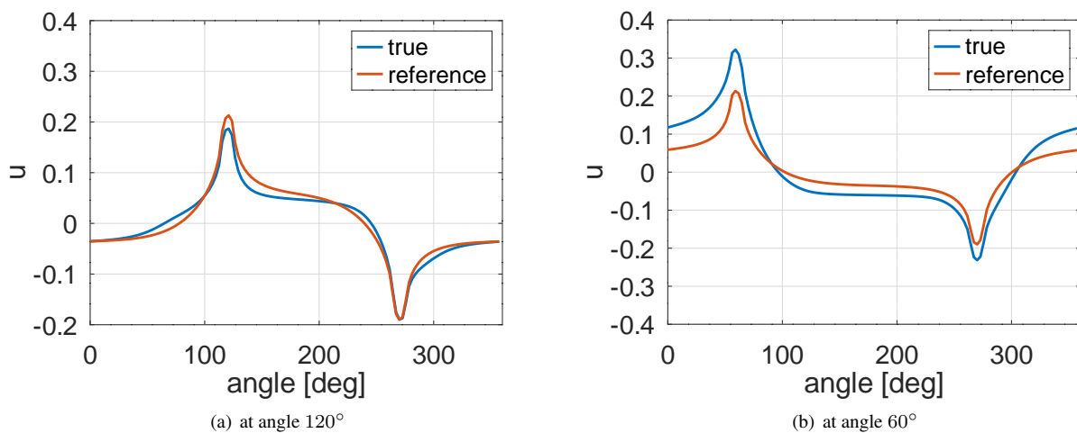
Figure 138: Voltage along the boundary
