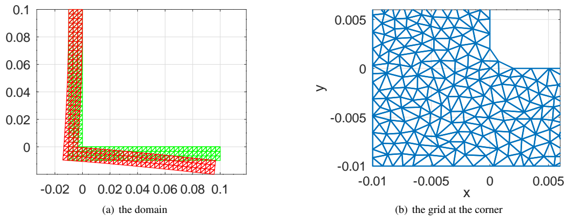
Figure 164: Original and deformed domain for the crook with attached weight at the right edge
