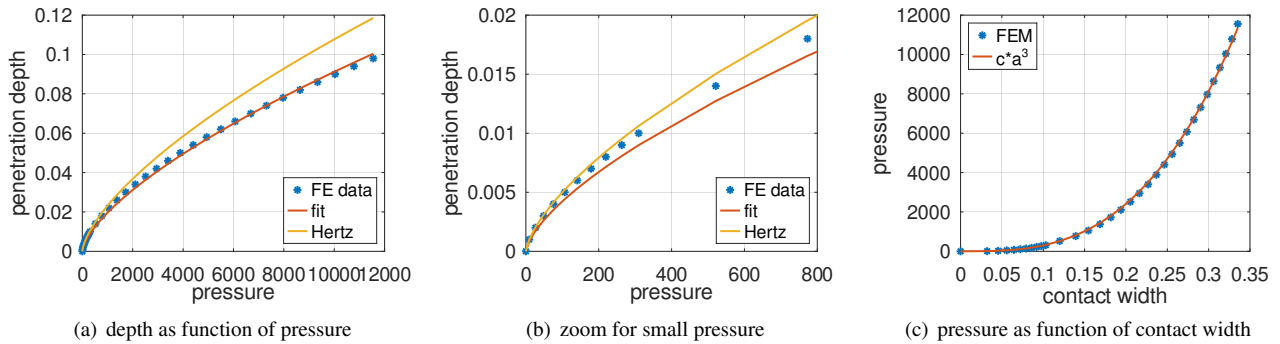
Figure 188: Contact with sphere: results of pressure and contact width for large penetration depth
