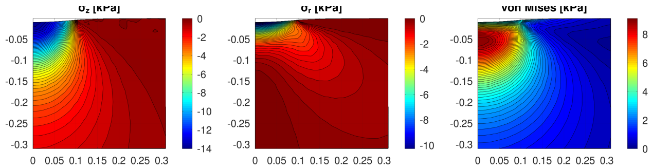
Figure 190: Contact with sphere: contours for the two normal stresses and the von Mises stress
