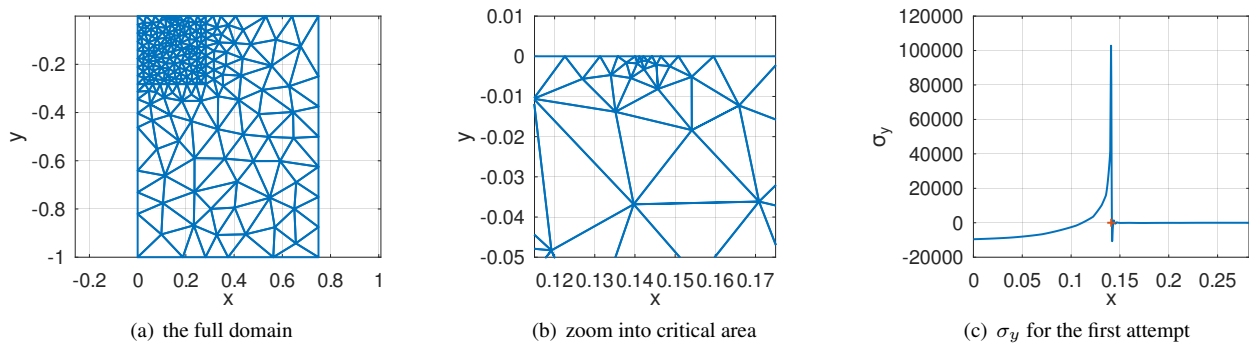
Figure 182: The mesh for the cylinder contact problem
